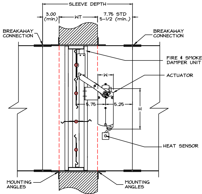
DOUBLE-SIDED MTG. ANGLES (EXTERNAL)
