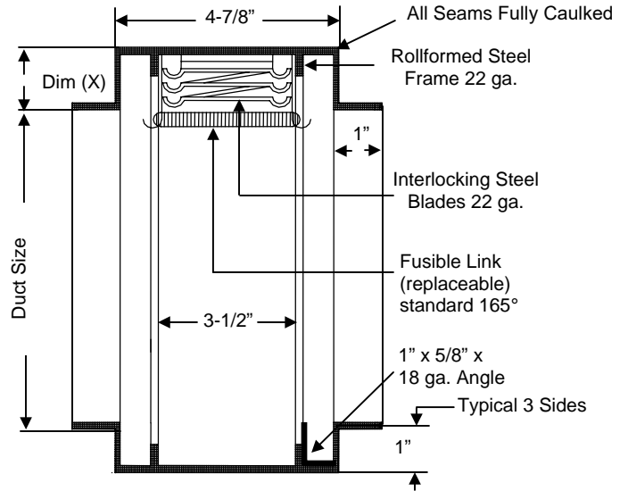
Vertical Section
