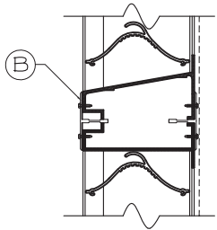
(B) HORIZONTAL VISIBLE MULLION
