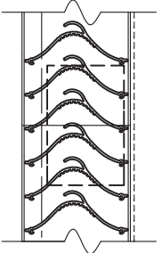
HORIZONTAL INVISIBLE MULLION
