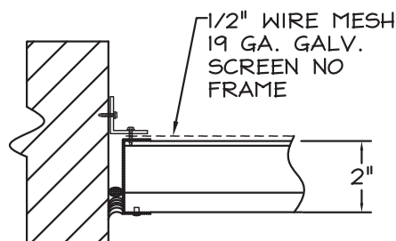
BOX FRAME
