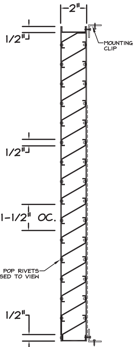
VERTICAL SECTION
